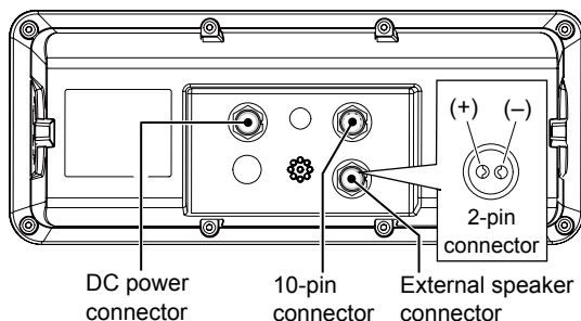
RC-M600's rear panel
